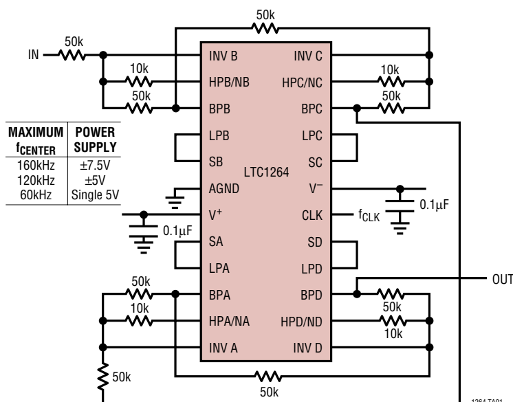
Clock-Tunable 8th Order Bandpass Filter, f_{\text{CENTER}} = f_{\text{CLK}}/20
