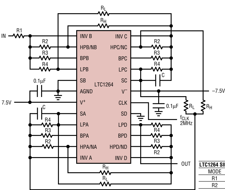
Clock-Tunable, 8th Order Elliptic Lowpass Filter, f_{CLK}/f_{CUTOFF} = 20:1
