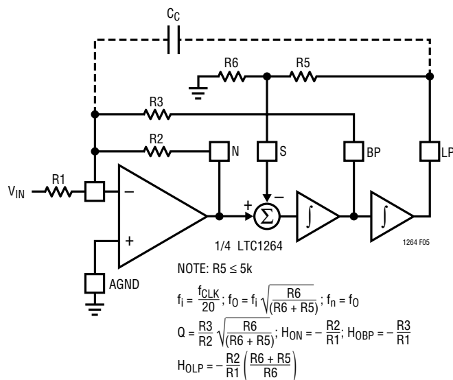
Figure 5. Mode 1b, 2nd Order Filter Providing Notch, Bandpass and Lowpass Outputs
